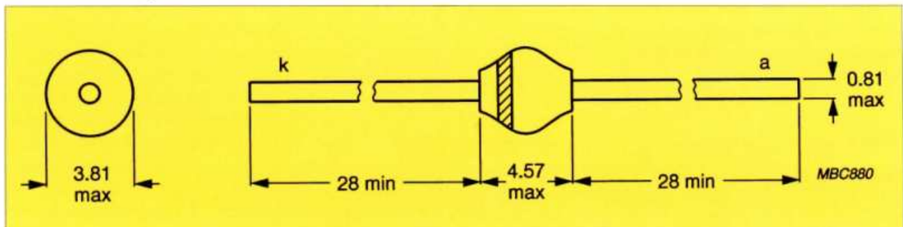
SOD-57-omhulling.
