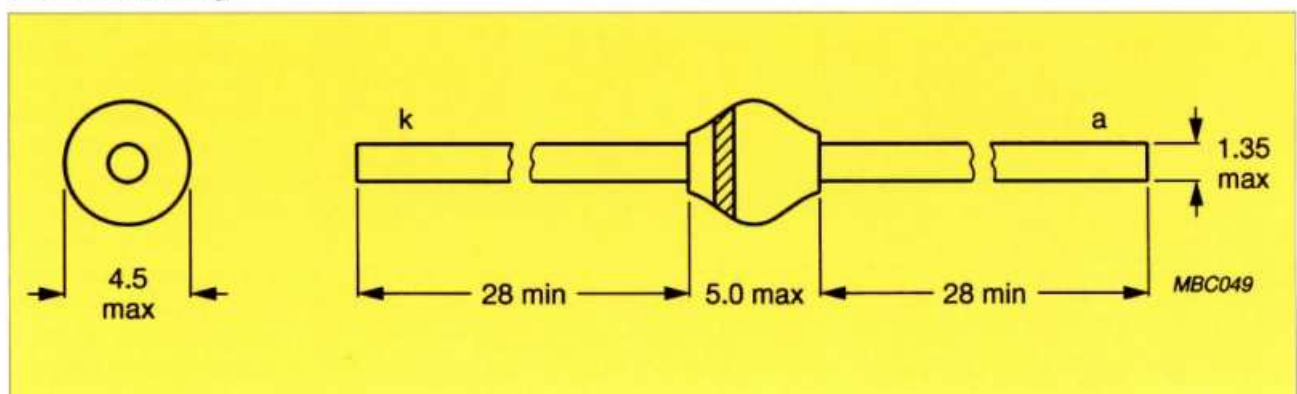
SOD-64-omhulling.
